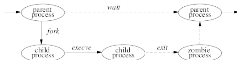
Figure 2.1. Process lifecycle
